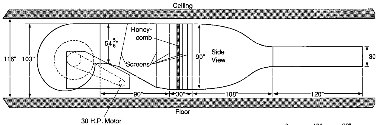
30 in. x 30 in. Blower Tunnel
