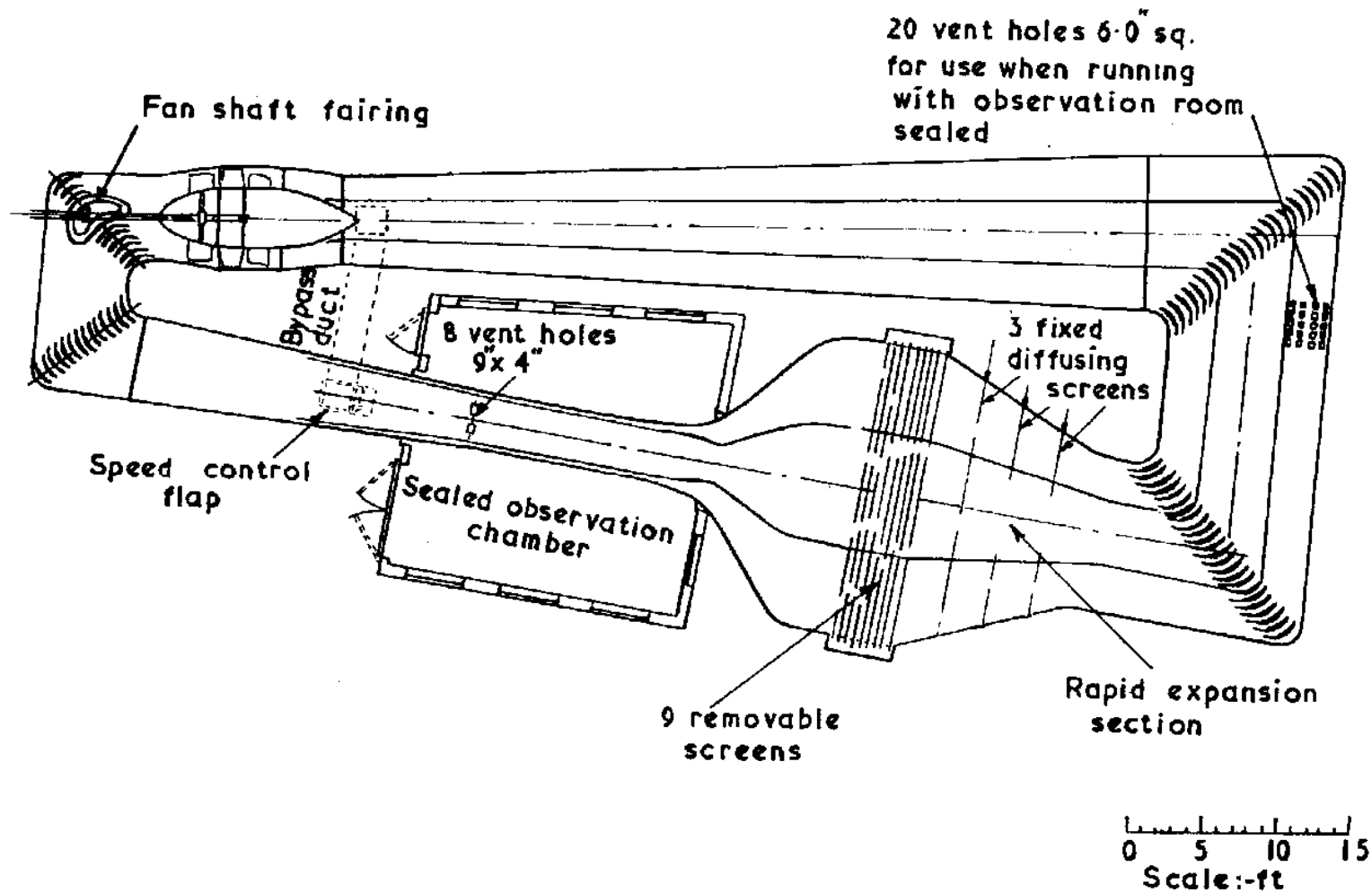
RAE 4 ft × 3 ft wind tunnel (1946).
