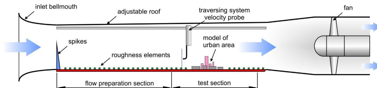
Sketch of a boundary layer wind tunnel
