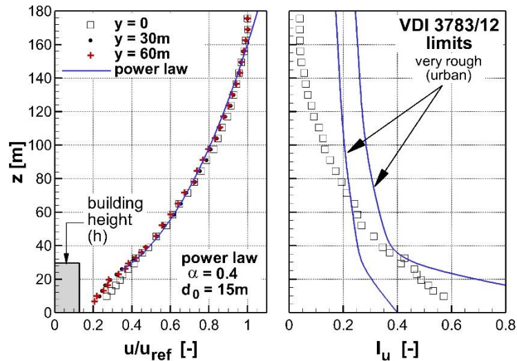
Left: vertical profiles of dimensionless mean velocity u_d of the approach flow at different offset distances from the symmetry plane ( y = 0 ). Right: vertical profile of turbulence intensity I_u in the symmetry plane. Dimensions given in full scale
