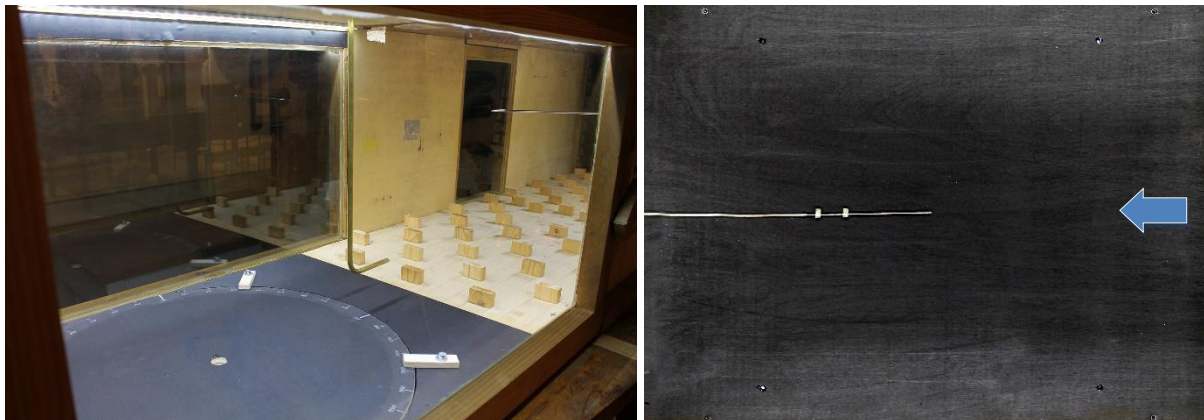
Left: LED lighting in the wind tunnel. right: Check of light homogeneity using a black painted plate in the test section. (Image contrast was increased to make the differences more visible)
