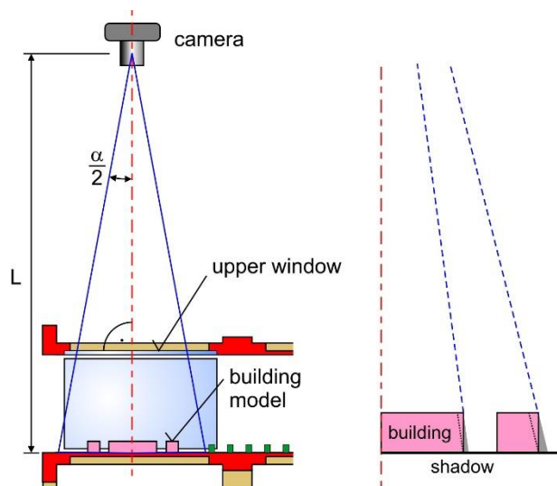
Left: the proper setup of the camera above the model. Right: blind spots due to vertical walls. Dotted lines show the slanted walls to remove the blind spots.
