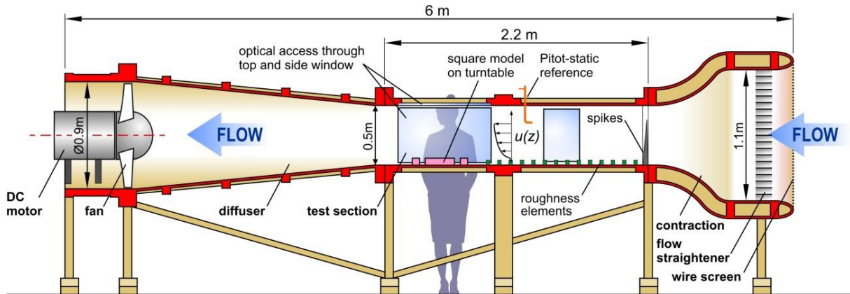
The NPL type wind tunnel with its main components, and the measurement setup with the boundary layer generating elements and the wind tunnel model placed in the test section.
