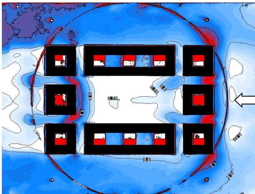
Resulting composite image of Velocity speed-up ratio (VSR) post processed by the Tecplot data visualisation software. Red areas indicate high-speed zones (VSR is high), white areas indicate low speeded zones (VSR is low)
