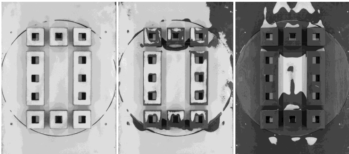
Left: wind tunnel model in initial state, covered with sand. Centre and right: sand removed from the model at small and higher wind tunnel speed.
