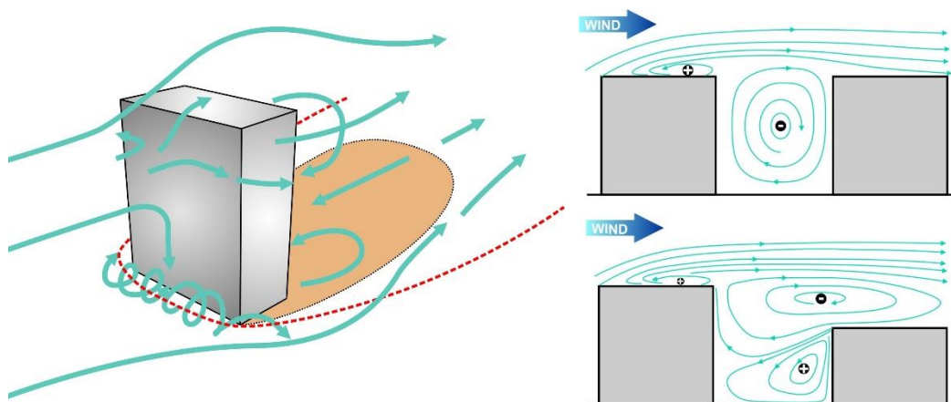
Flow field around a tall building (Beranek and van Koten) Street canyons of different buildings.
