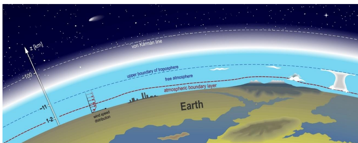
A schematic view of the atmospheric boundary layer
