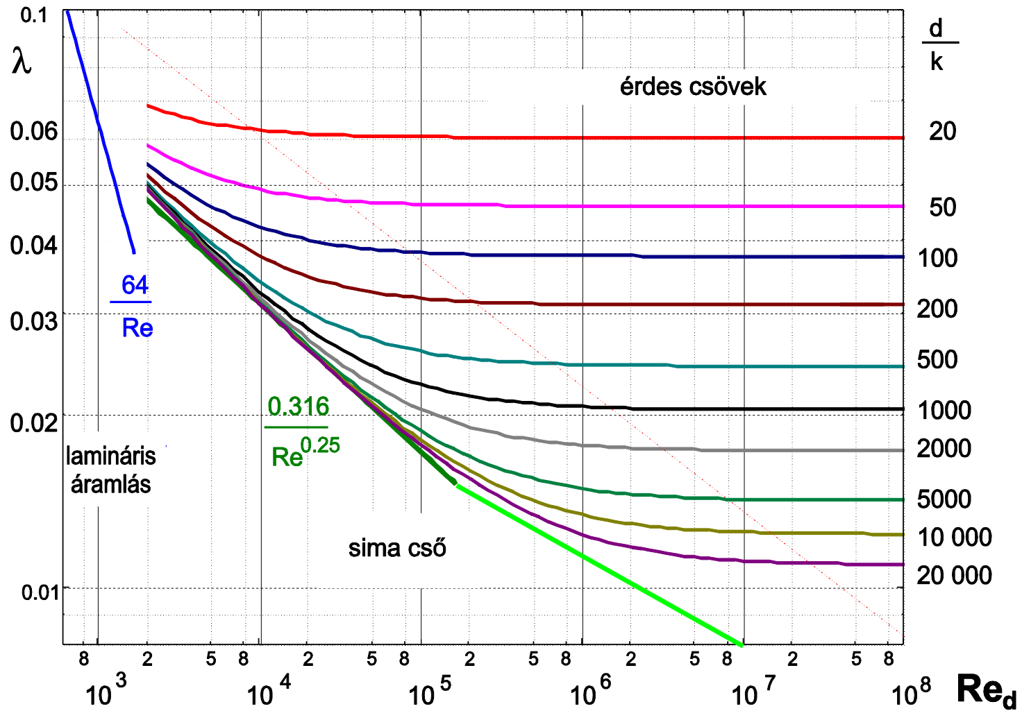
Moody-diagram
